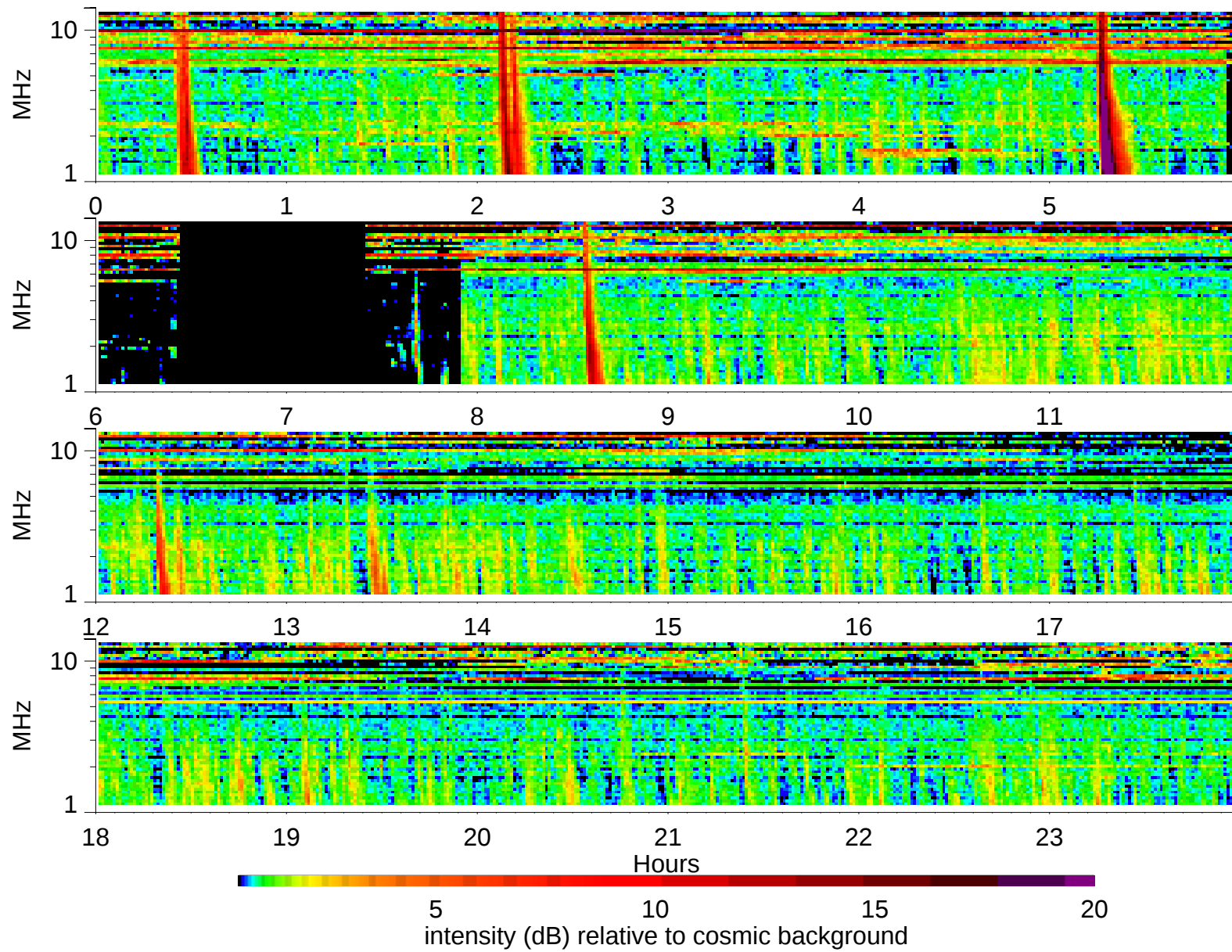
Wind Waves RAD2 receiver: 1997/9/12
