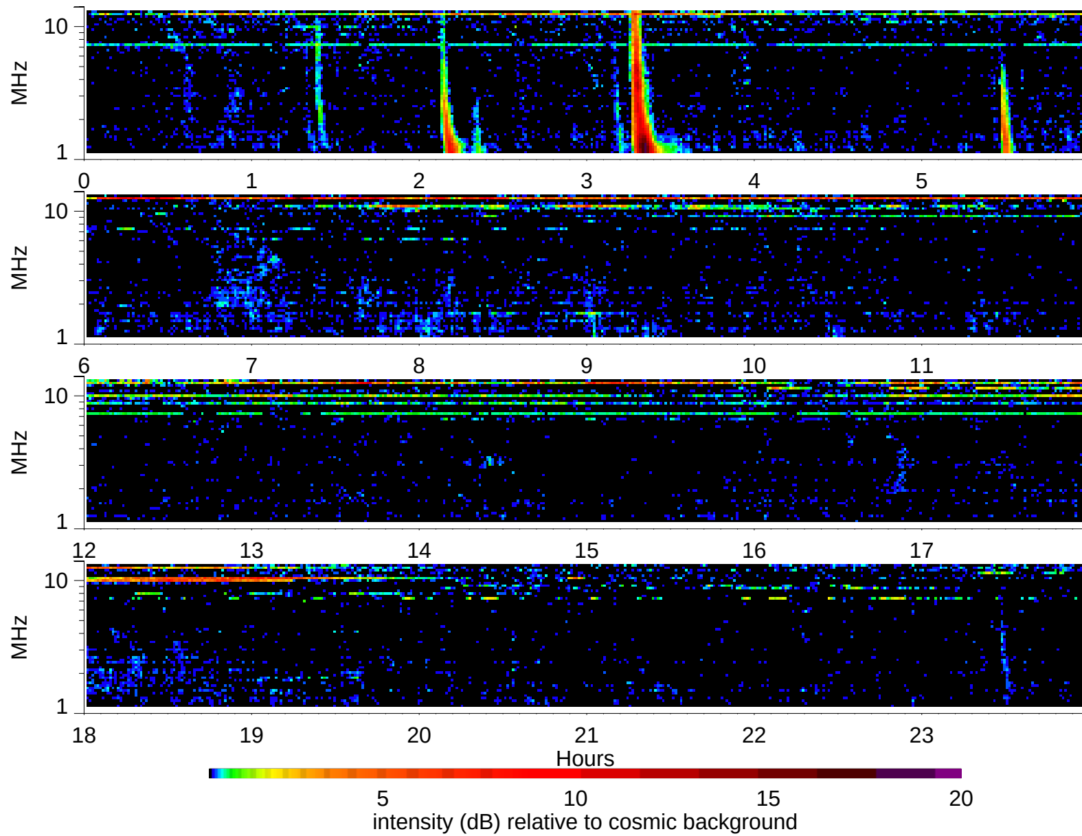
Wind Waves RAD2 receiver: 1997/9/20
