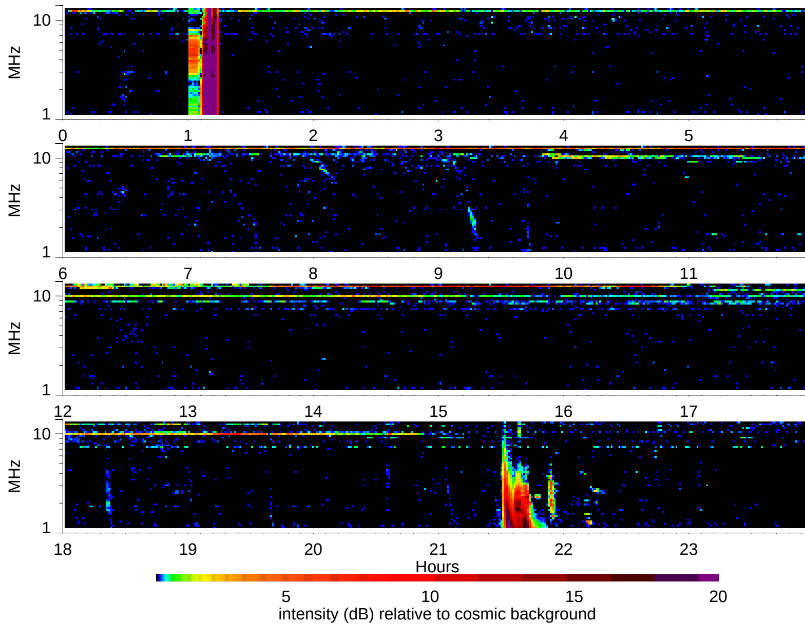
Wind Waves RAD2 receiver: 1997/9/23
