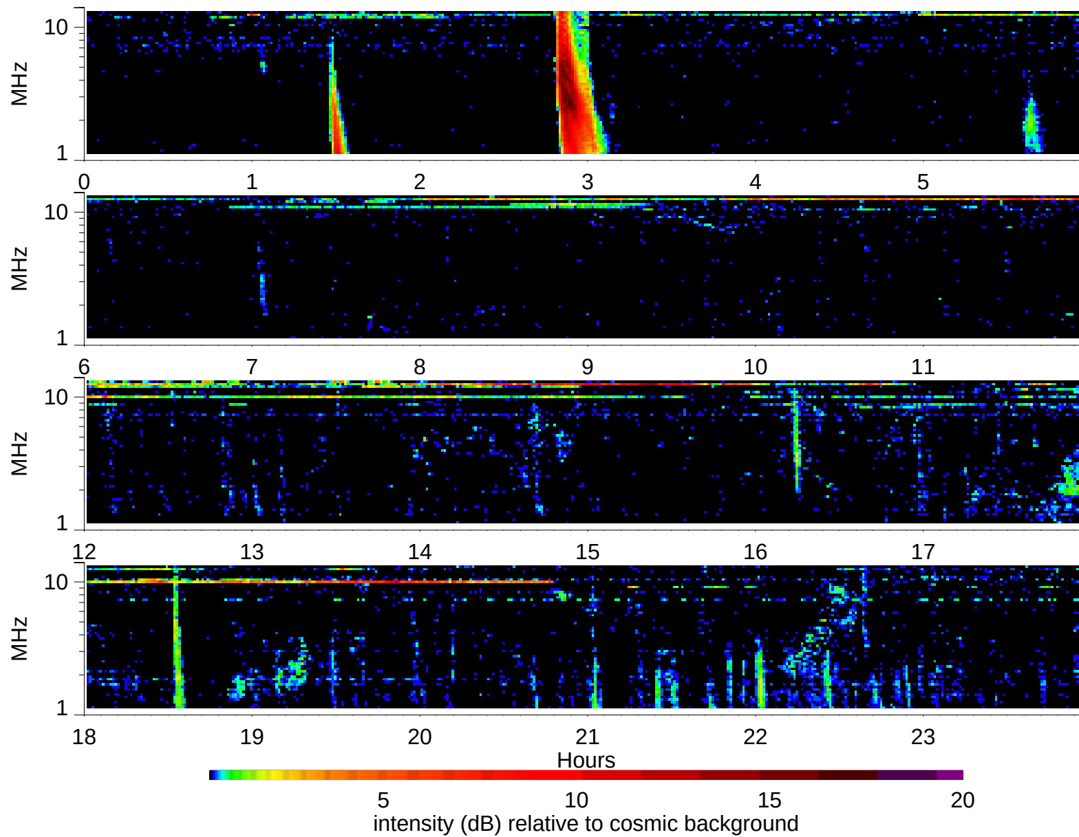
Wind Waves RAD2 receiver: 1997/9/24
