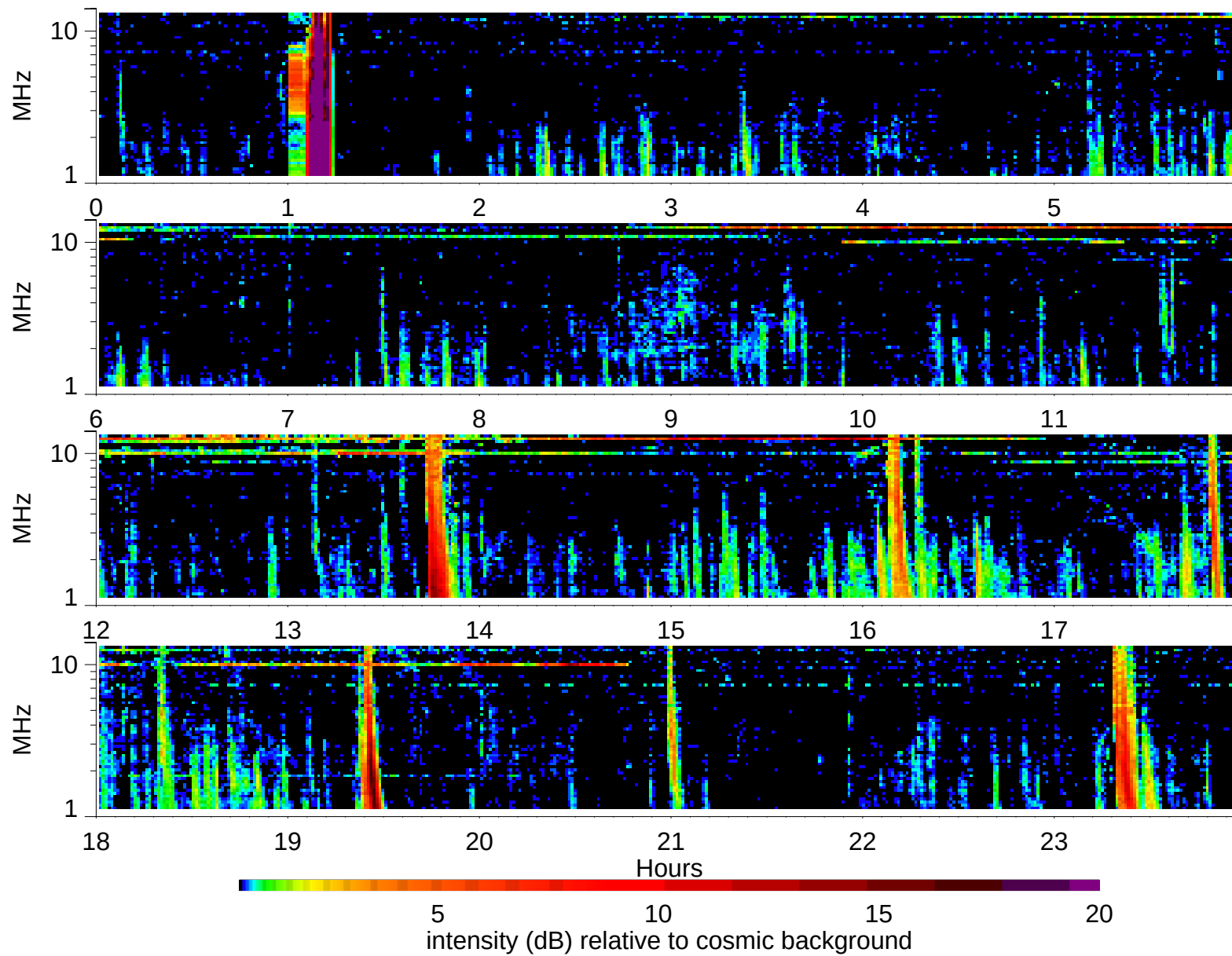
Wind Waves RAD2 receiver: 1997/9/25
