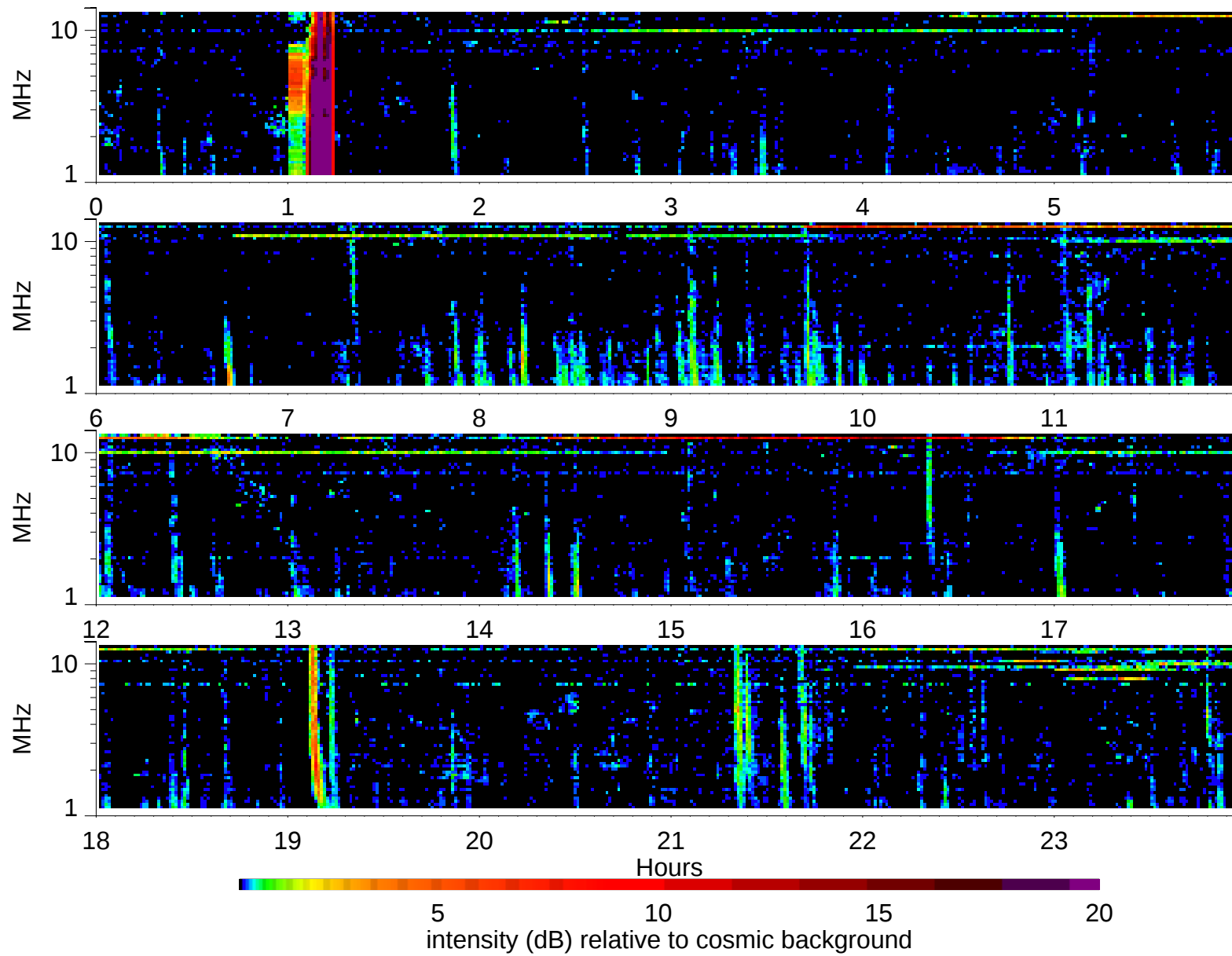
Wind Waves RAD2 receiver: 1997/9/27
