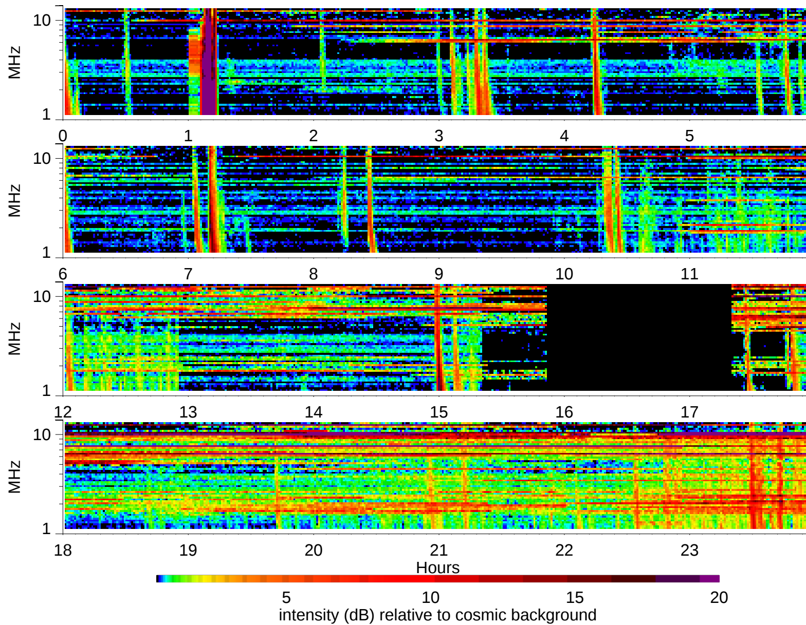
Wind Waves RAD2 receiver: 1997/9/29
