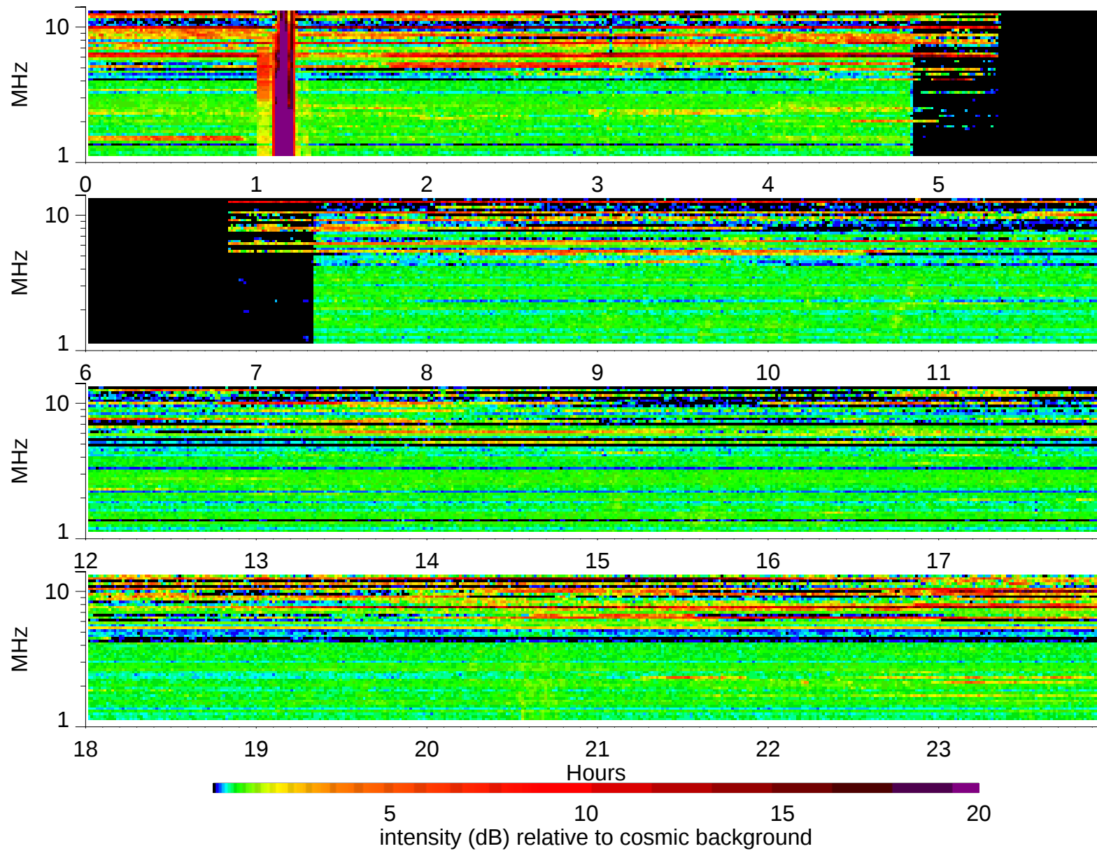
Wind Waves RAD2 receiver: 1997/10/3
