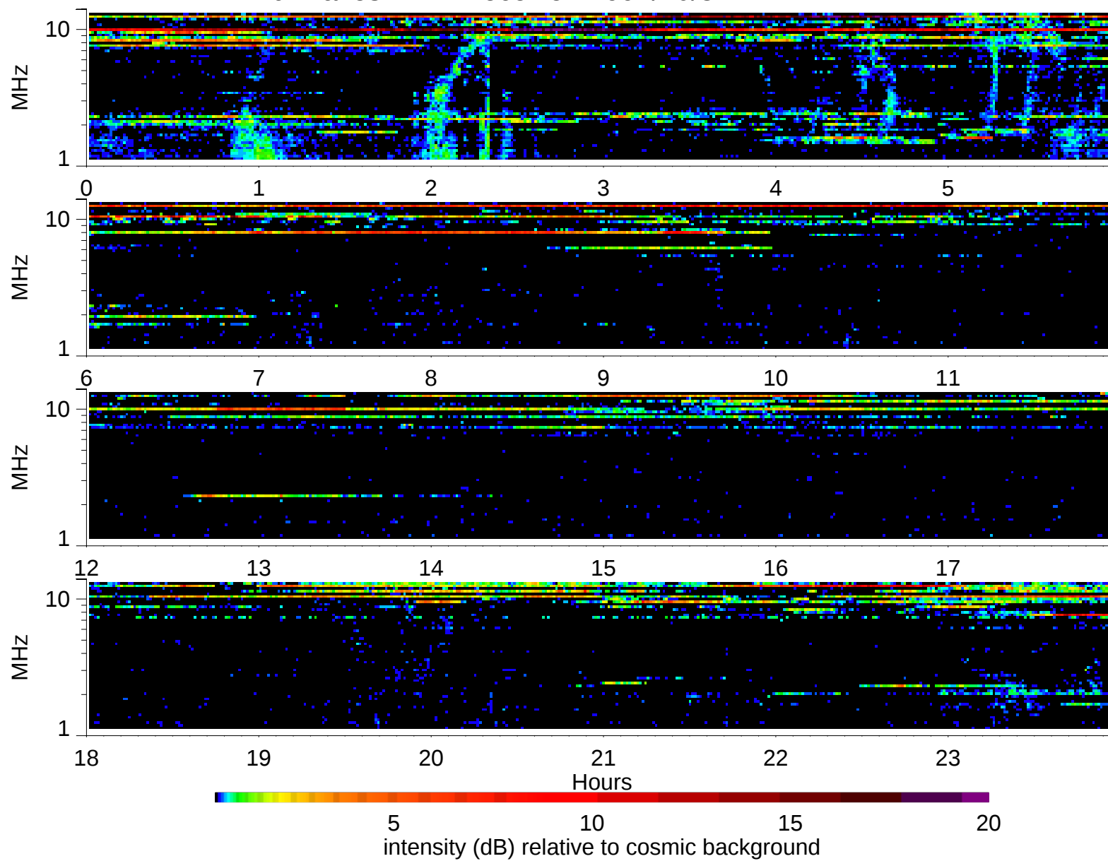
Wind Waves RAD2 receiver: 1997/10/8
