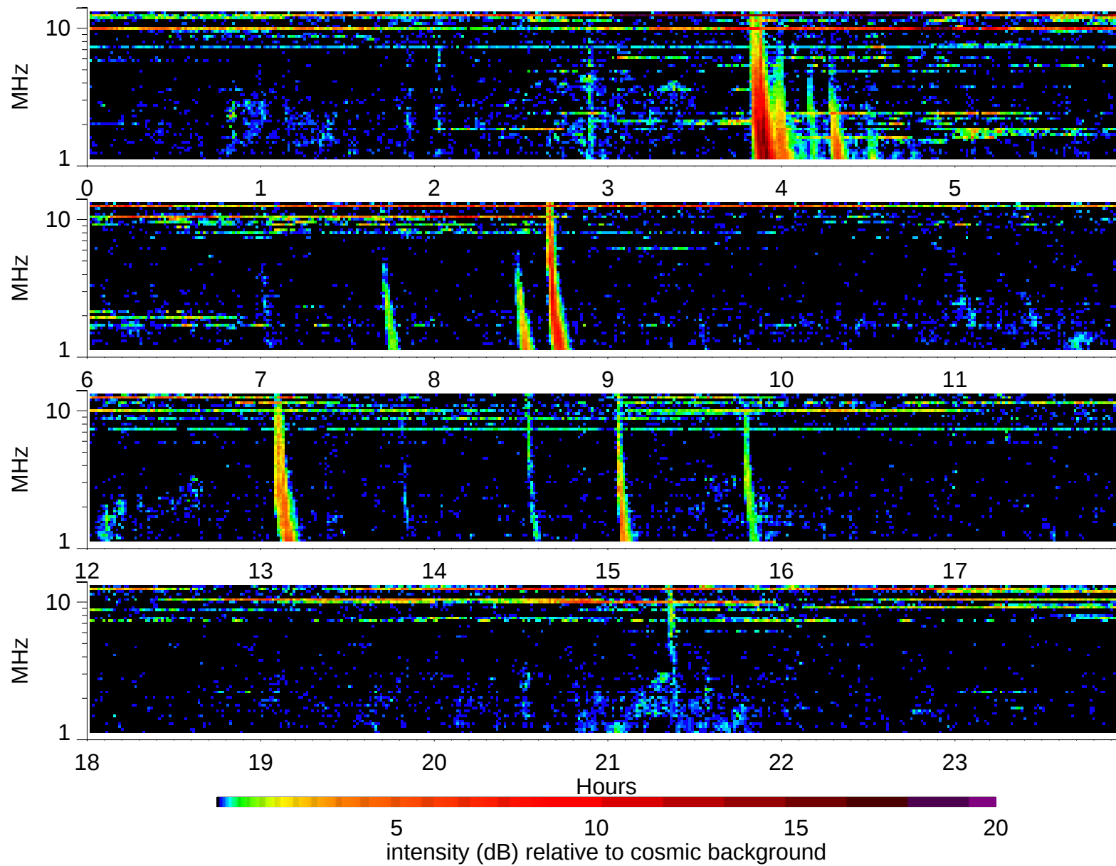
Wind Waves RAD2 receiver: 1997/10/10
