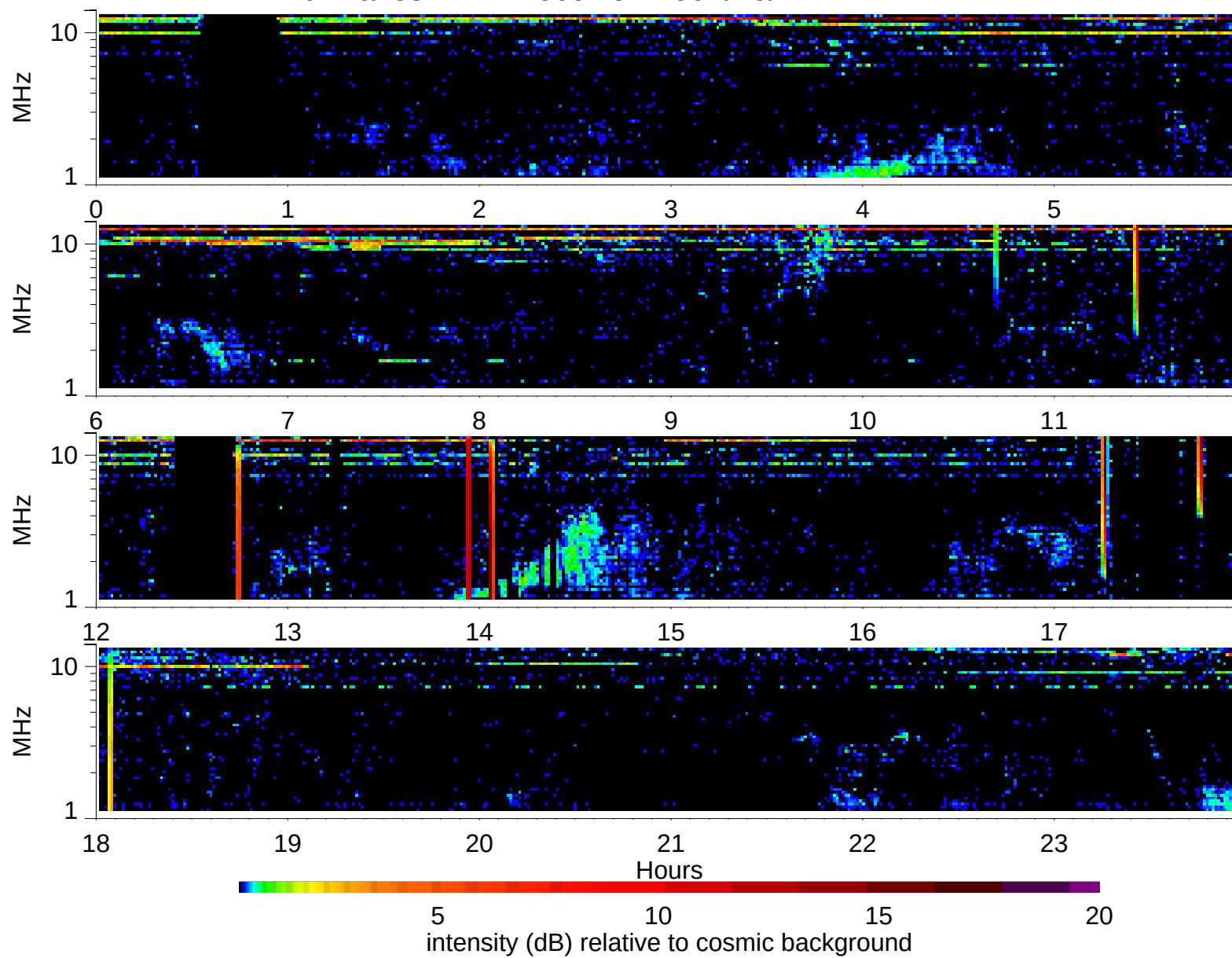
Wind Waves RAD2 receiver: 1997/10/12
