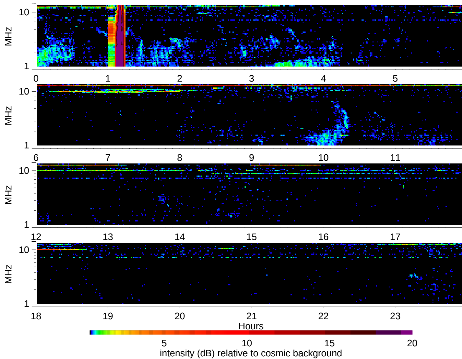
Wind Waves RAD2 receiver: 1997/10/13
