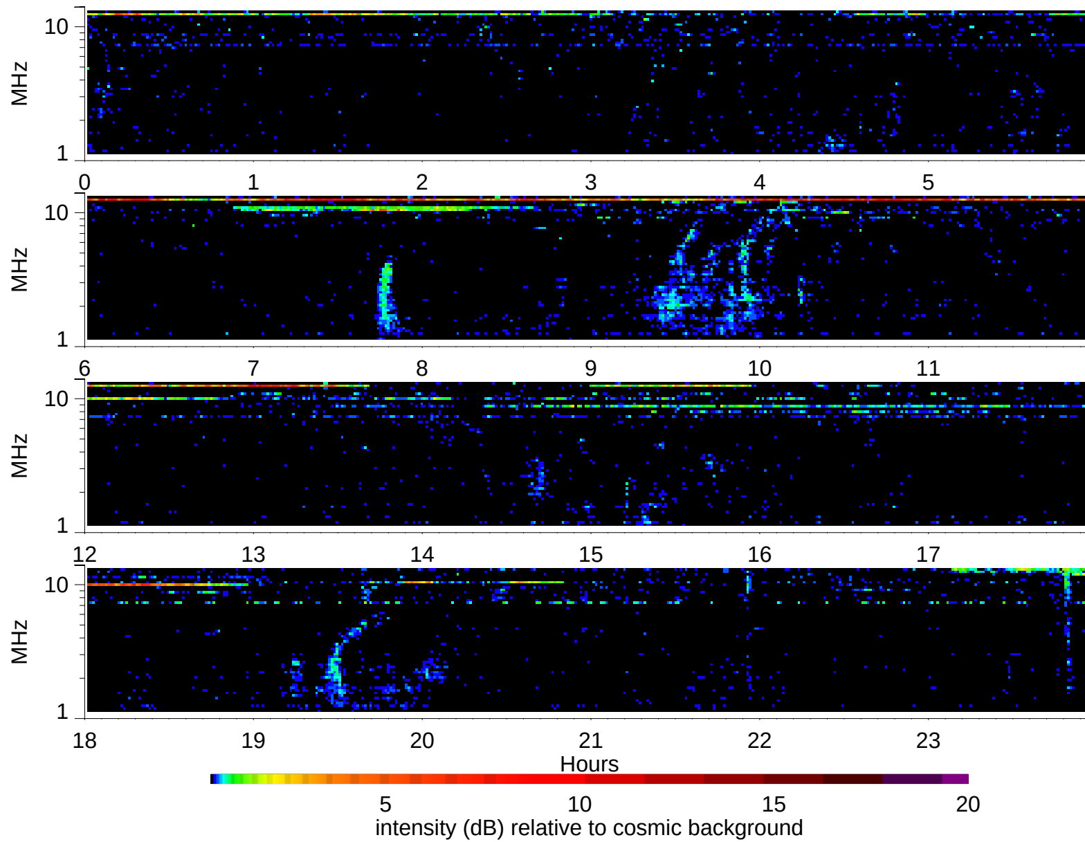
Wind Waves RAD2 receiver: 1997/10/14
