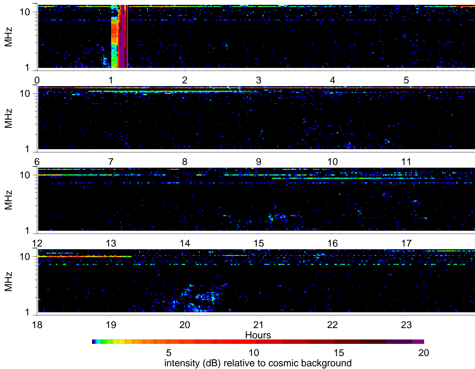
Wind Waves RAD2 receiver: 1997/10/15
