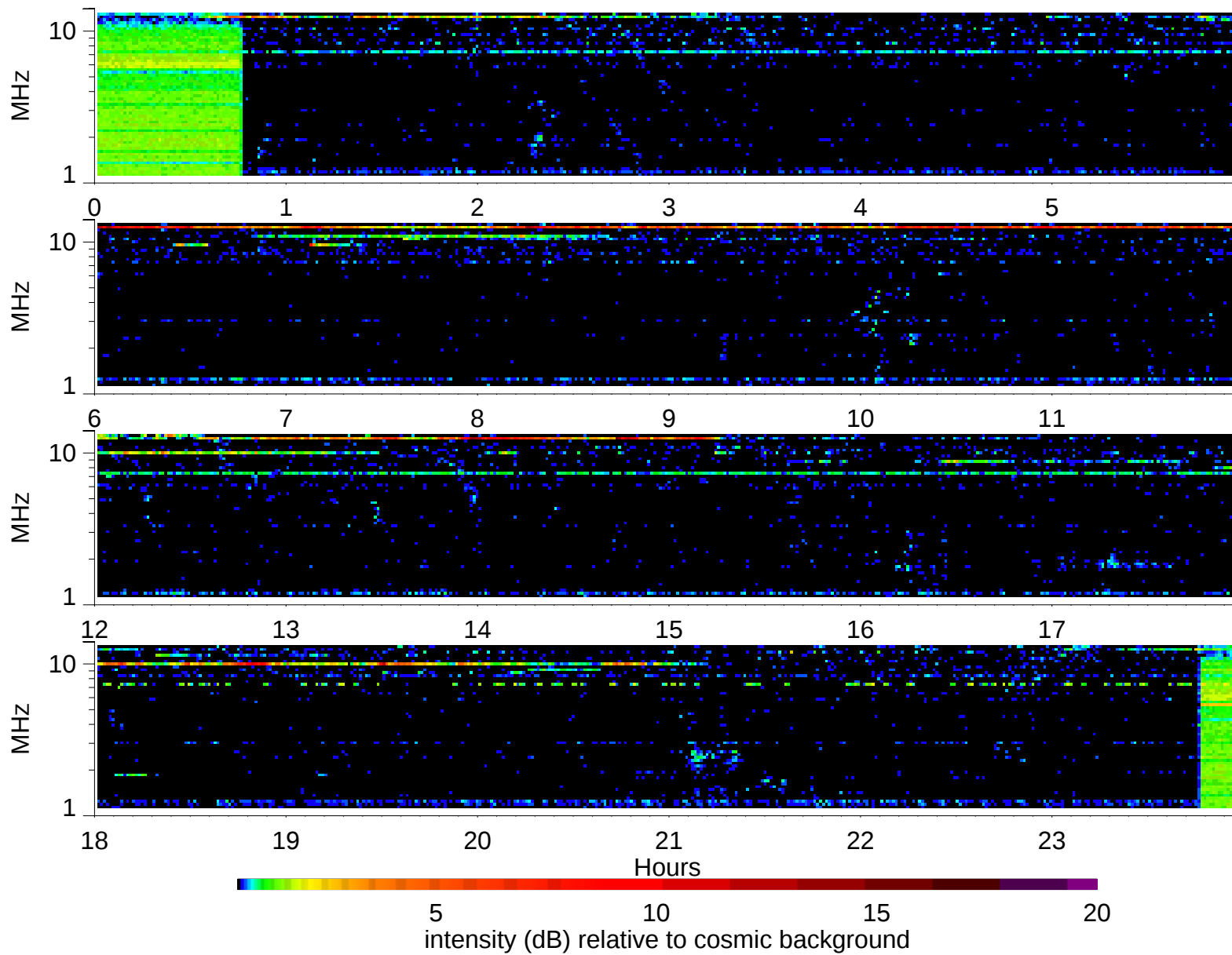
Wind Waves RAD2 receiver: 1997/10/16
