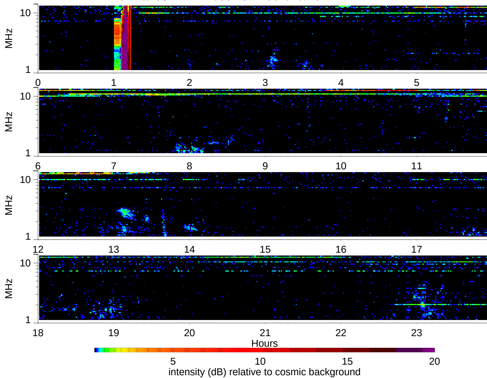
Wind Waves RAD2 receiver: 1997/10/19
