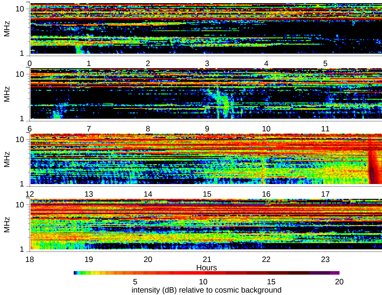
Wind Waves RAD2 receiver: 1997/10/21
