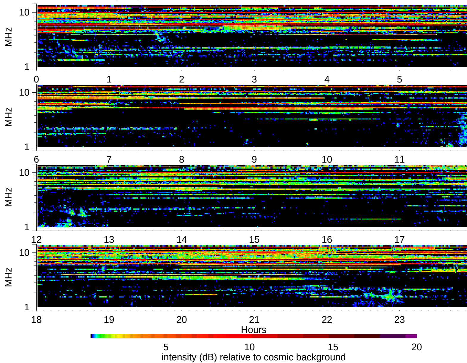
Wind Waves RAD2 receiver: 1997/10/24
