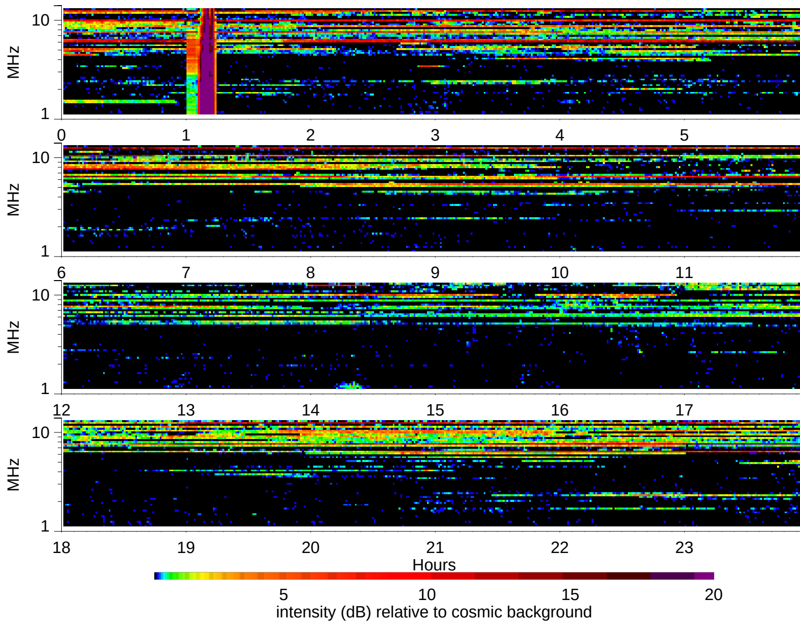
Wind Waves RAD2 receiver: 1997/10/25
