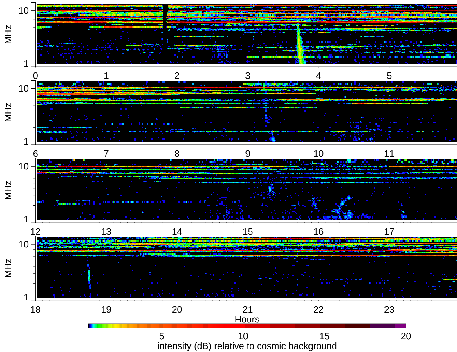
Wind Waves RAD2 receiver: 1997/10/28
