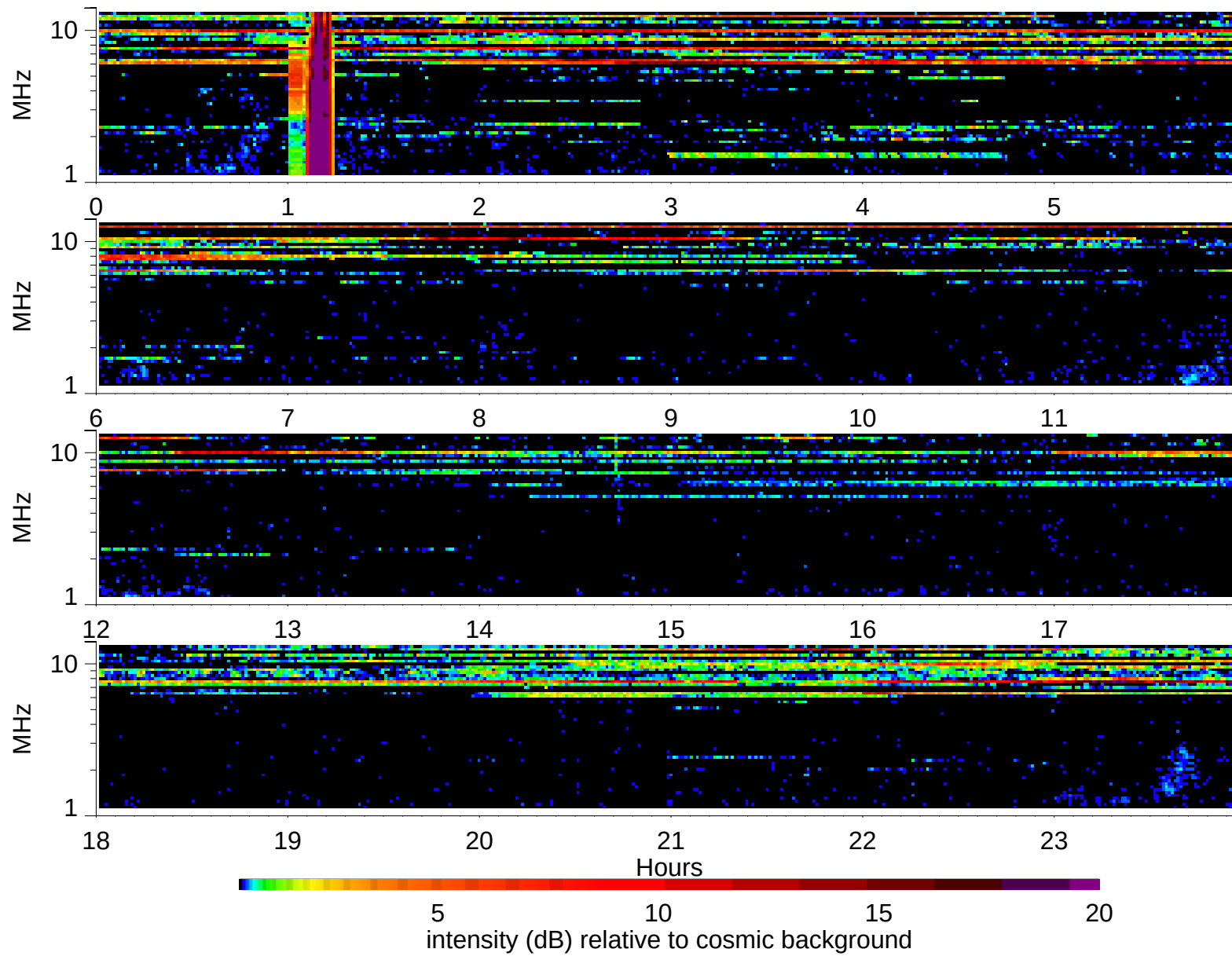
Wind Waves RAD2 receiver: 1997/10/29
