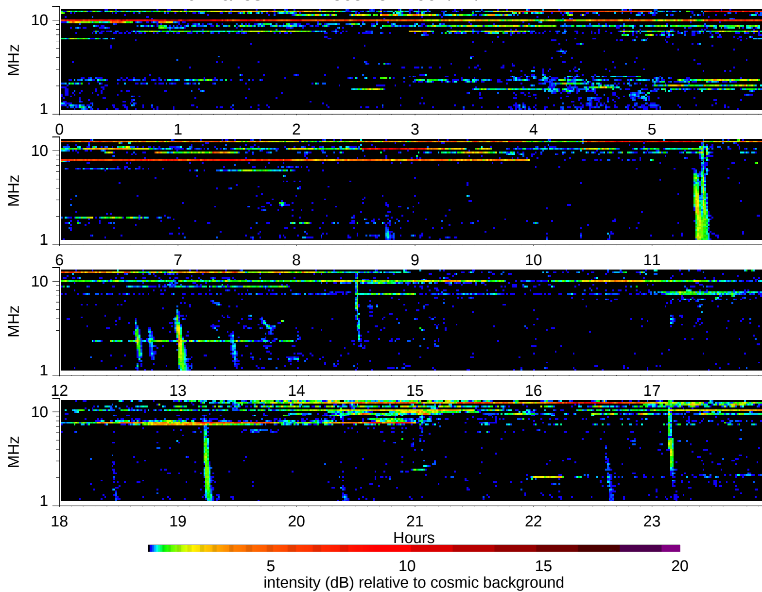
Wind Waves RAD2 receiver: 1997/11/1
