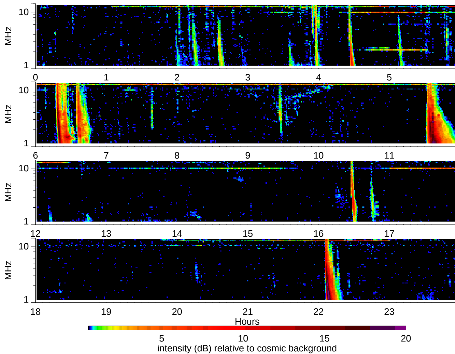
Wind Waves RAD2 receiver: 1997/11/5
