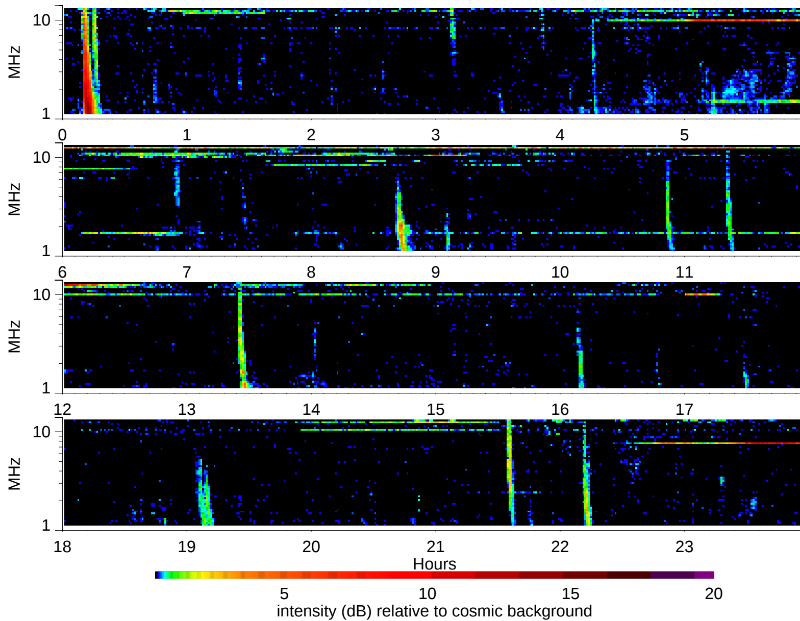
Wind Waves RAD2 receiver: 1997/11/7
