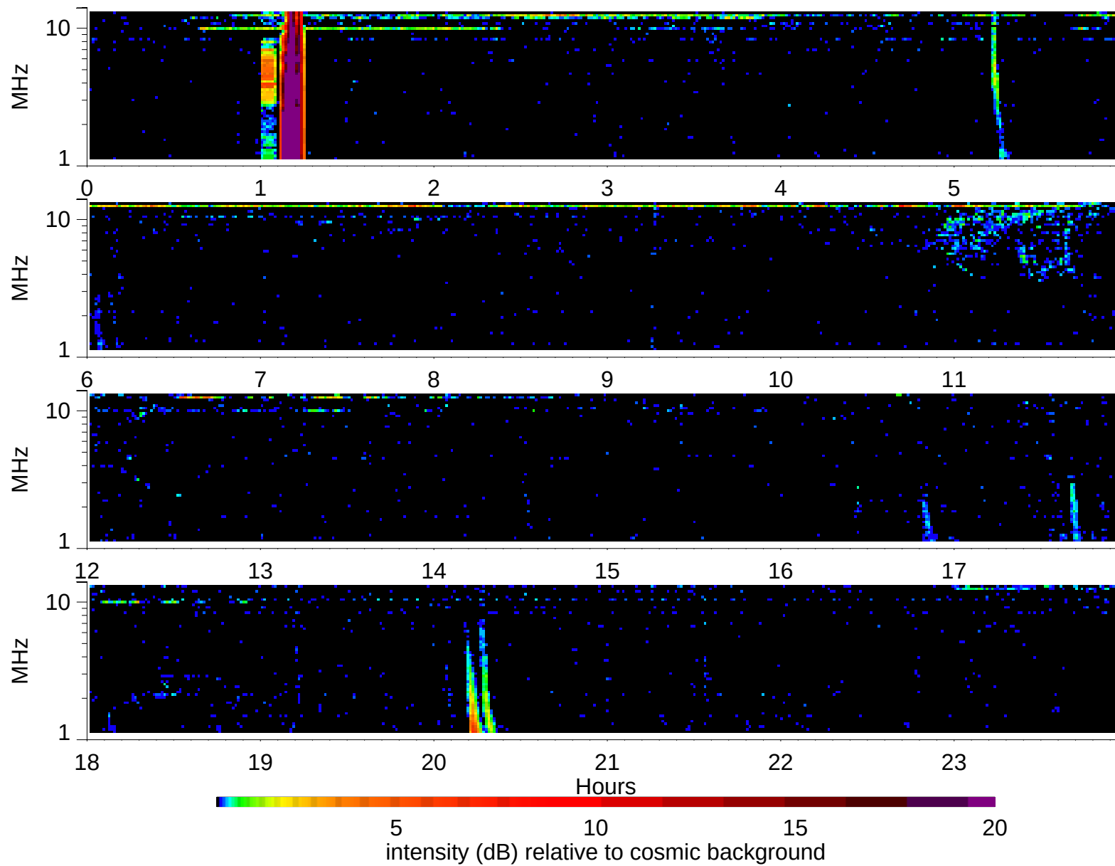
Wind Waves RAD2 receiver: 1997/11/12
