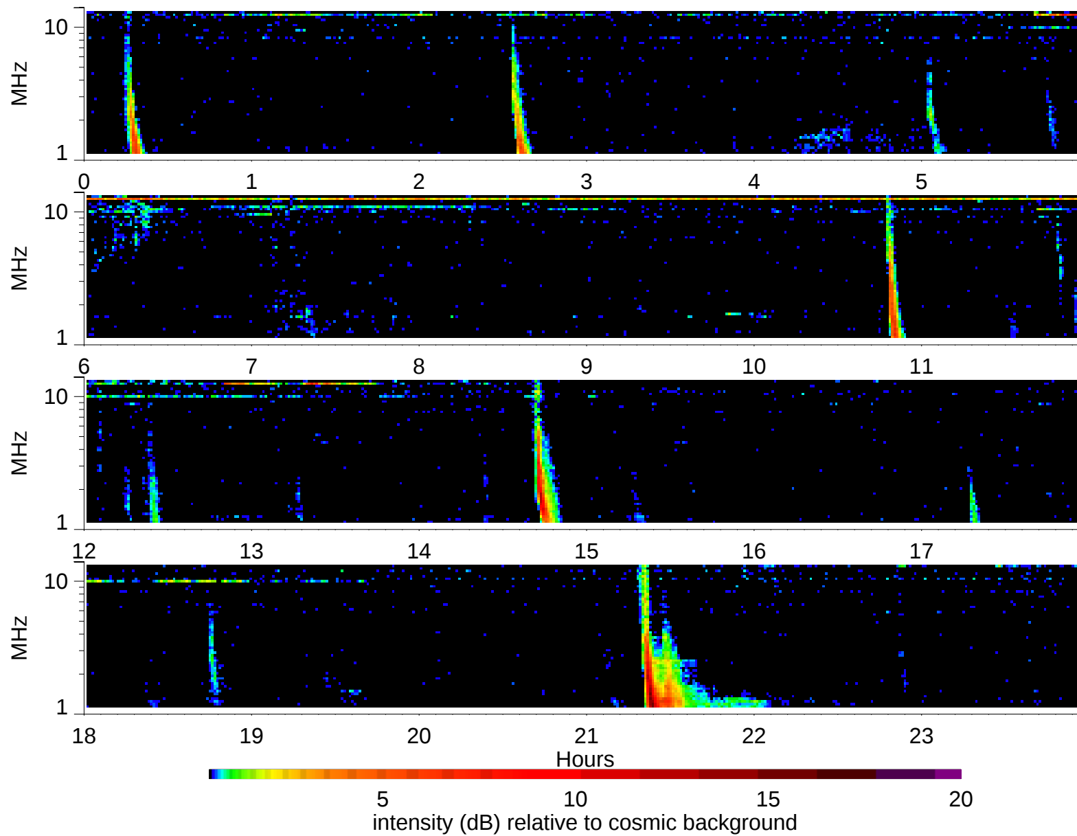
Wind Waves RAD2 receiver: 1997/11/13
