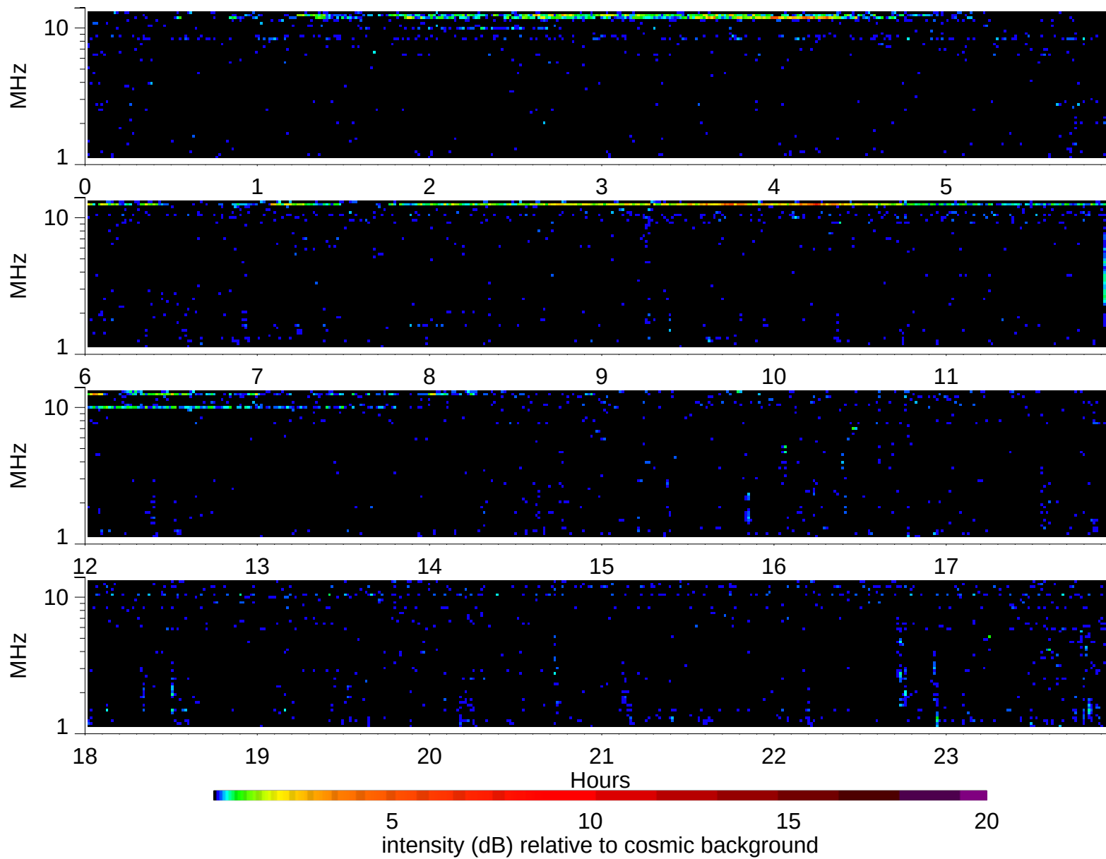
Wind Waves RAD2 receiver: 1997/11/15
