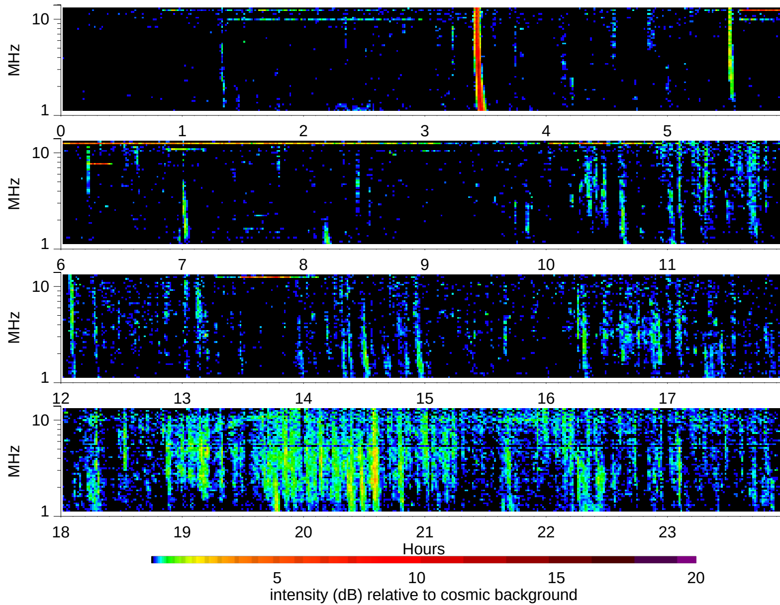
Wind Waves RAD2 receiver: 1997/11/17
