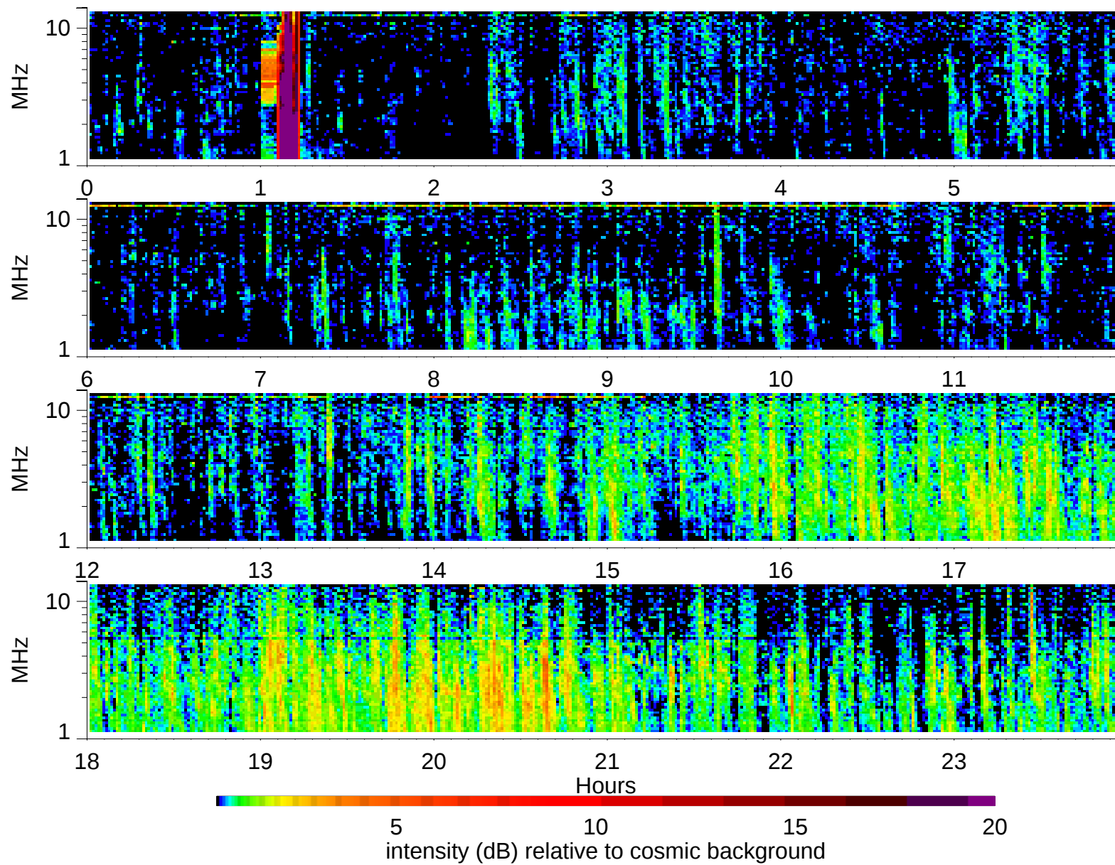
Wind Waves RAD2 receiver: 1997/11/18
