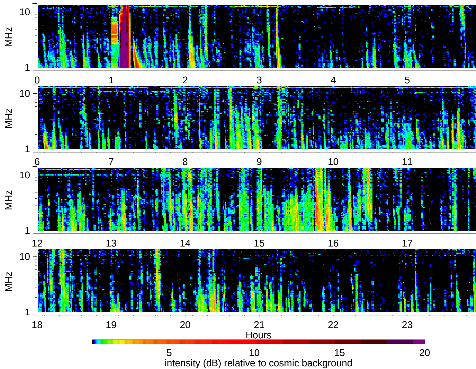
Wind Waves RAD2 receiver: 1997/11/20
