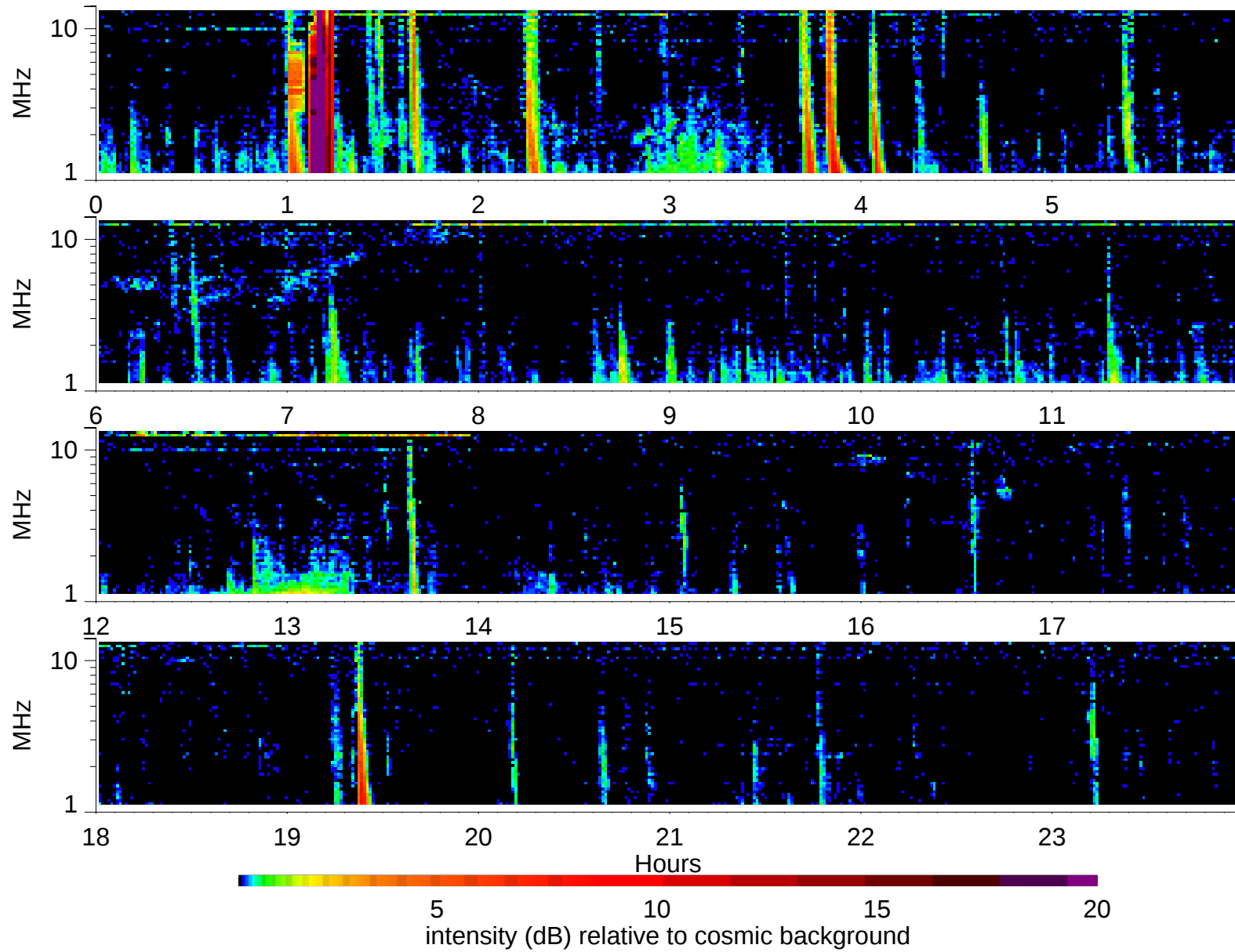
Wind Waves RAD2 receiver: 1997/11/22
