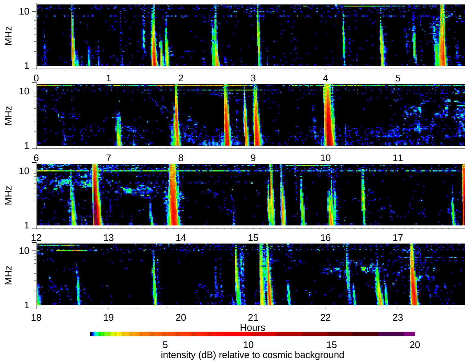
Wind Waves RAD2 receiver: 1997/11/23
