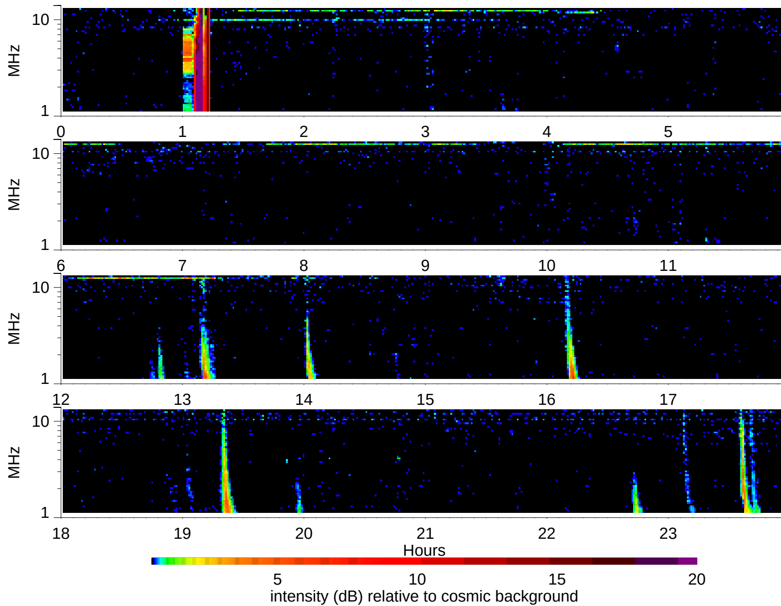
Wind Waves RAD2 receiver: 1997/11/26
