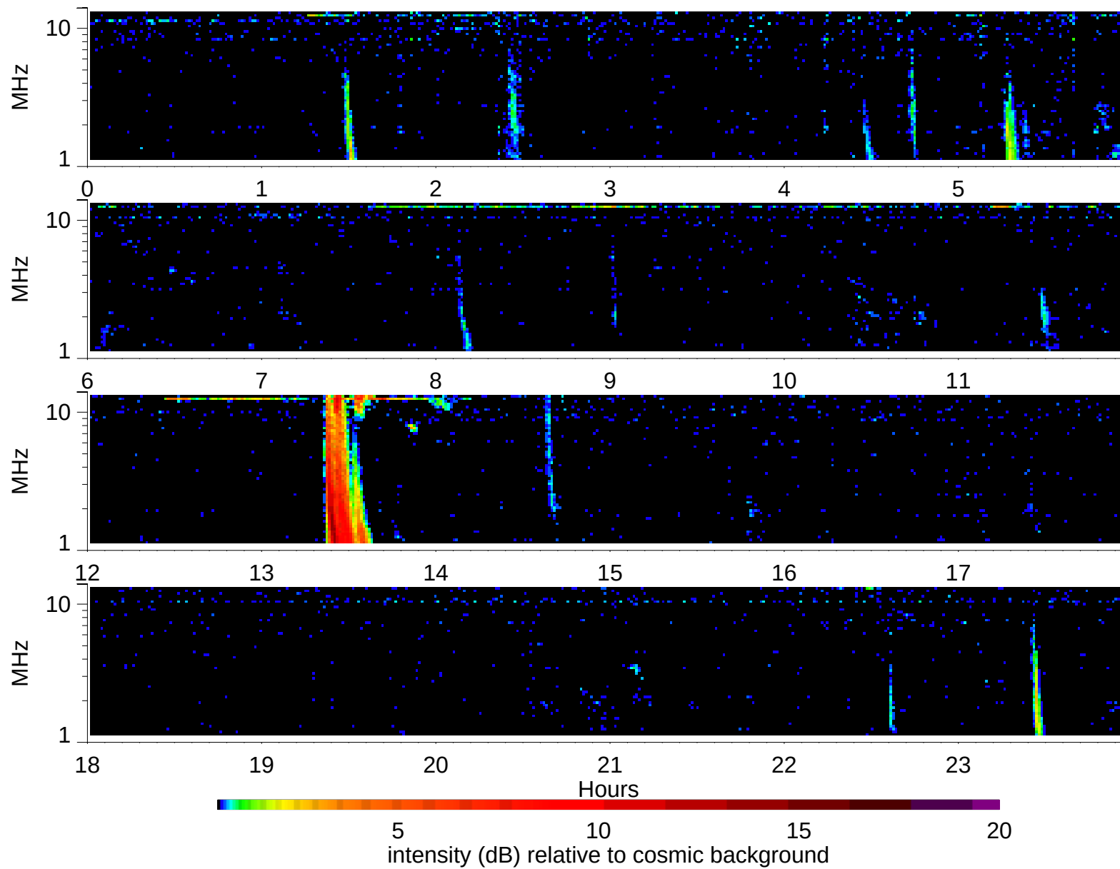
Wind Waves RAD2 receiver: 1997/11/27
