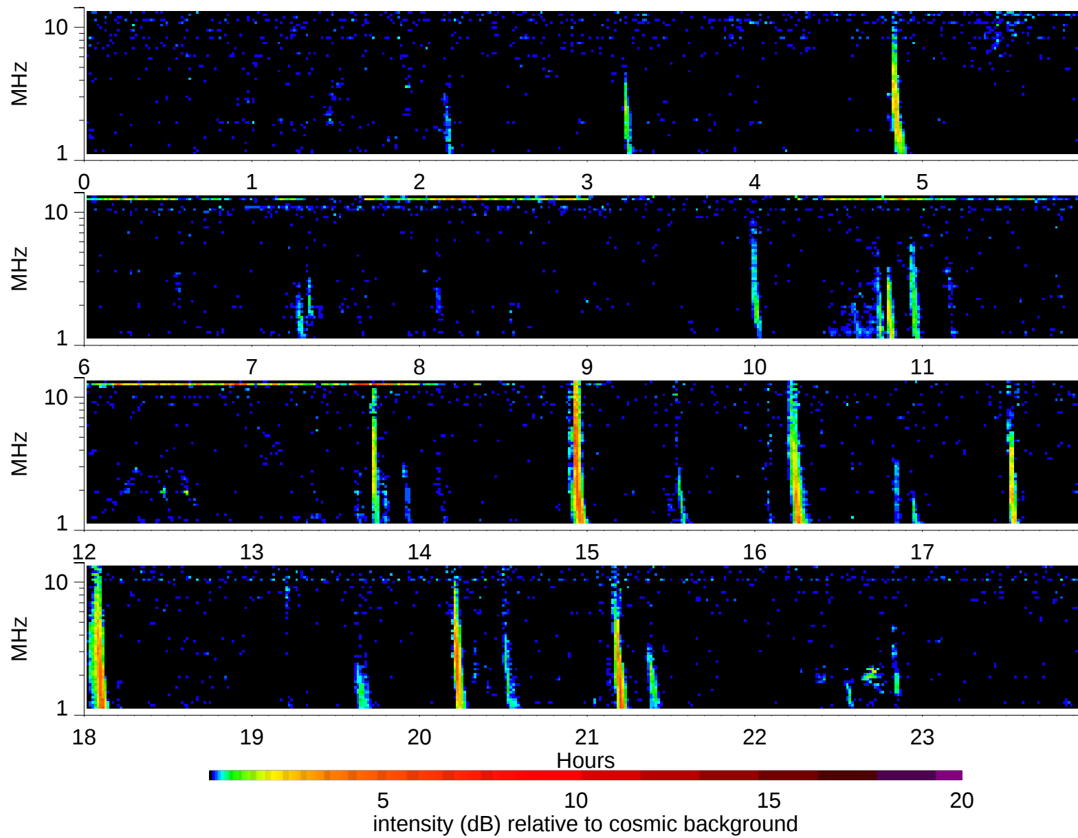
Wind Waves RAD2 receiver: 1997/11/29
