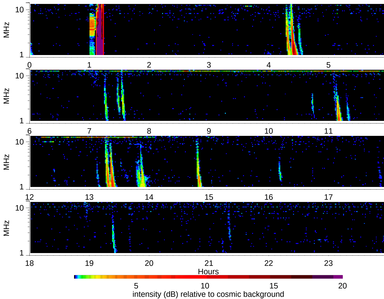
Wind Waves RAD2 receiver: 1997/12/6
