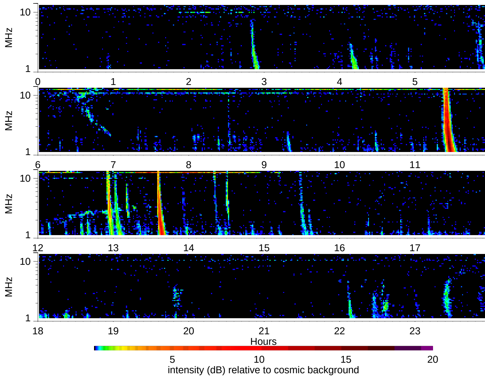
Wind Waves RAD2 receiver: 1997/12/7
