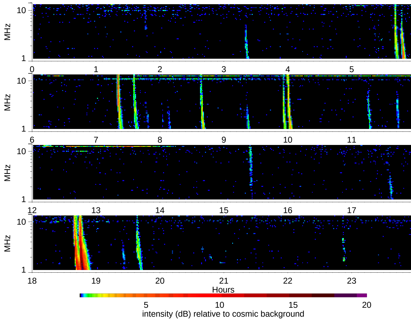
Wind Waves RAD2 receiver: 1997/12/9
