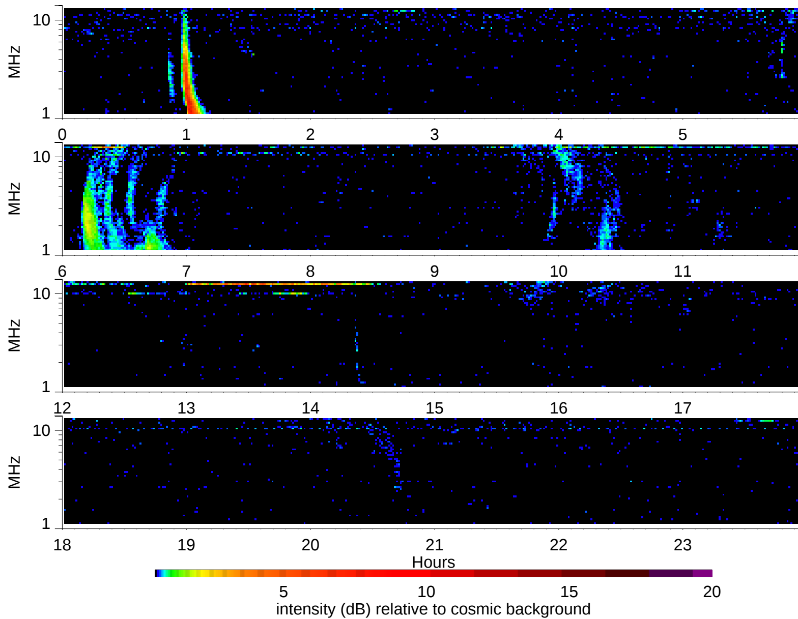
Wind Waves RAD2 receiver: 1997/12/13
