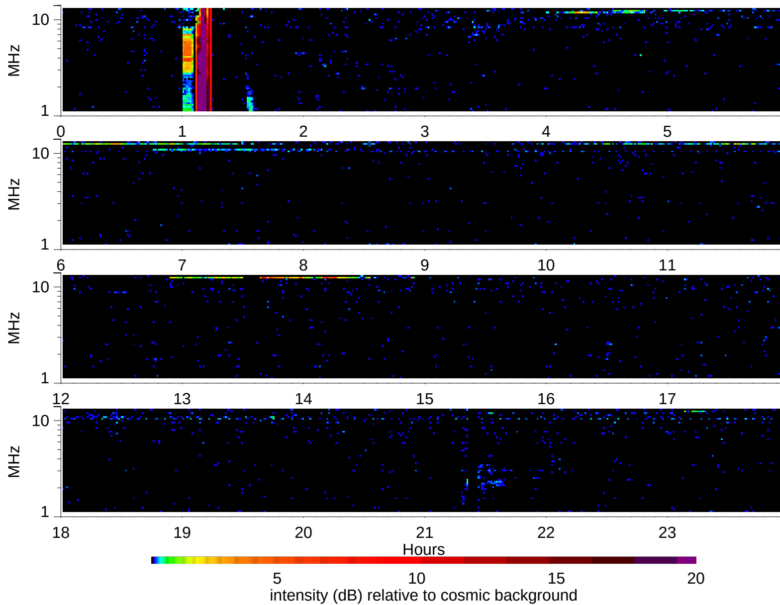
Wind Waves RAD2 receiver: 1997/12/22
