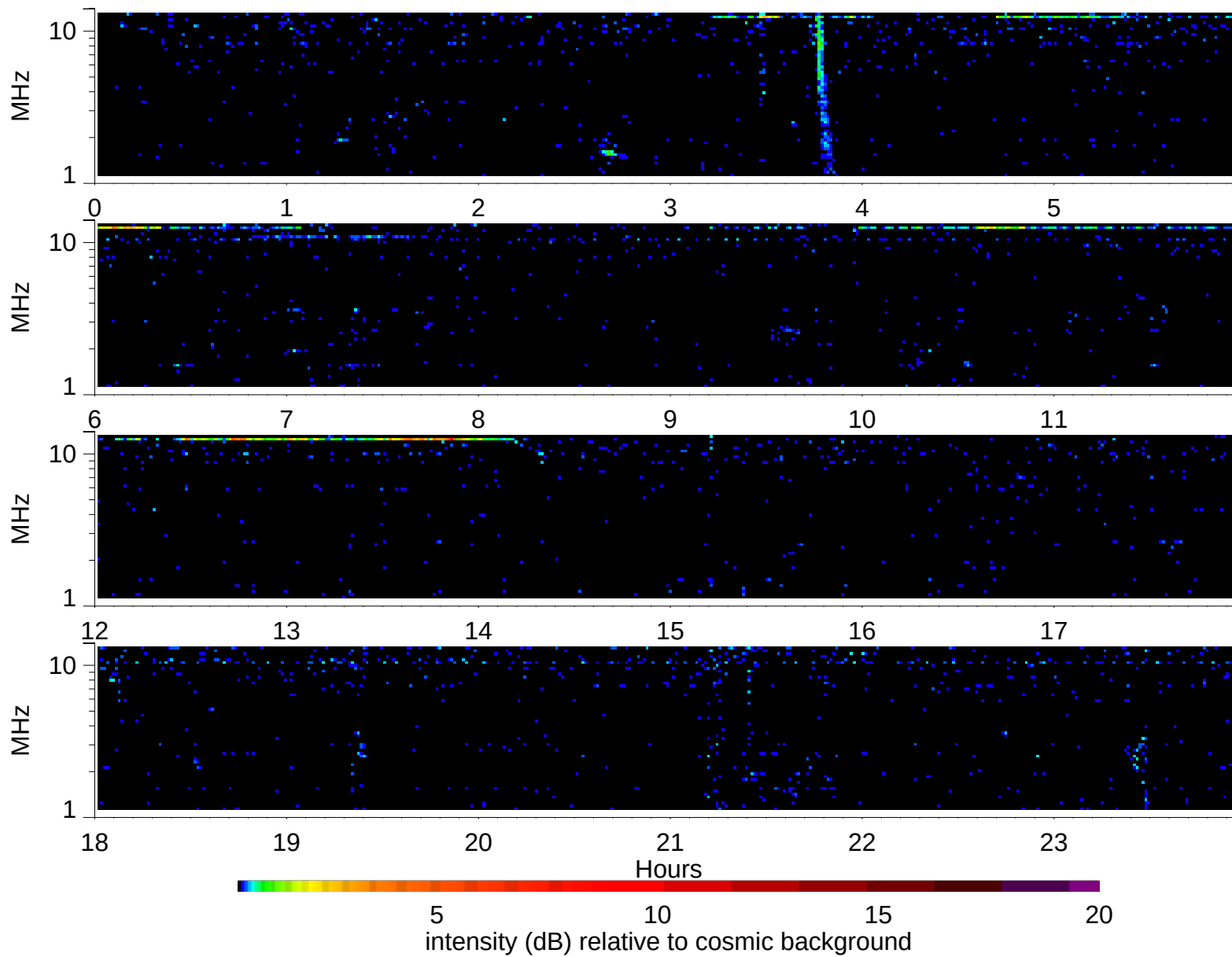
Wind Waves RAD2 receiver: 1997/12/23
