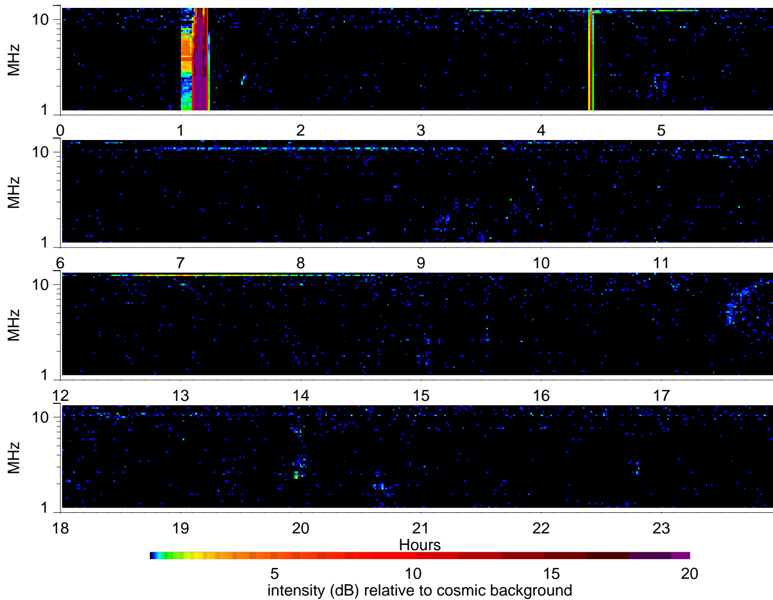
Wind Waves RAD2 receiver: 1997/12/26
