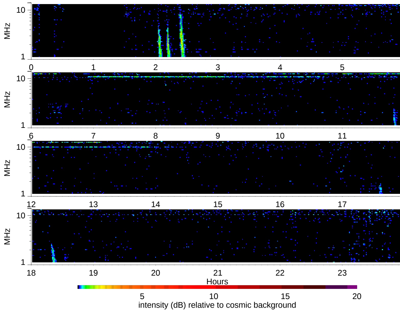
Wind Waves RAD2 receiver: 1998/1/5
