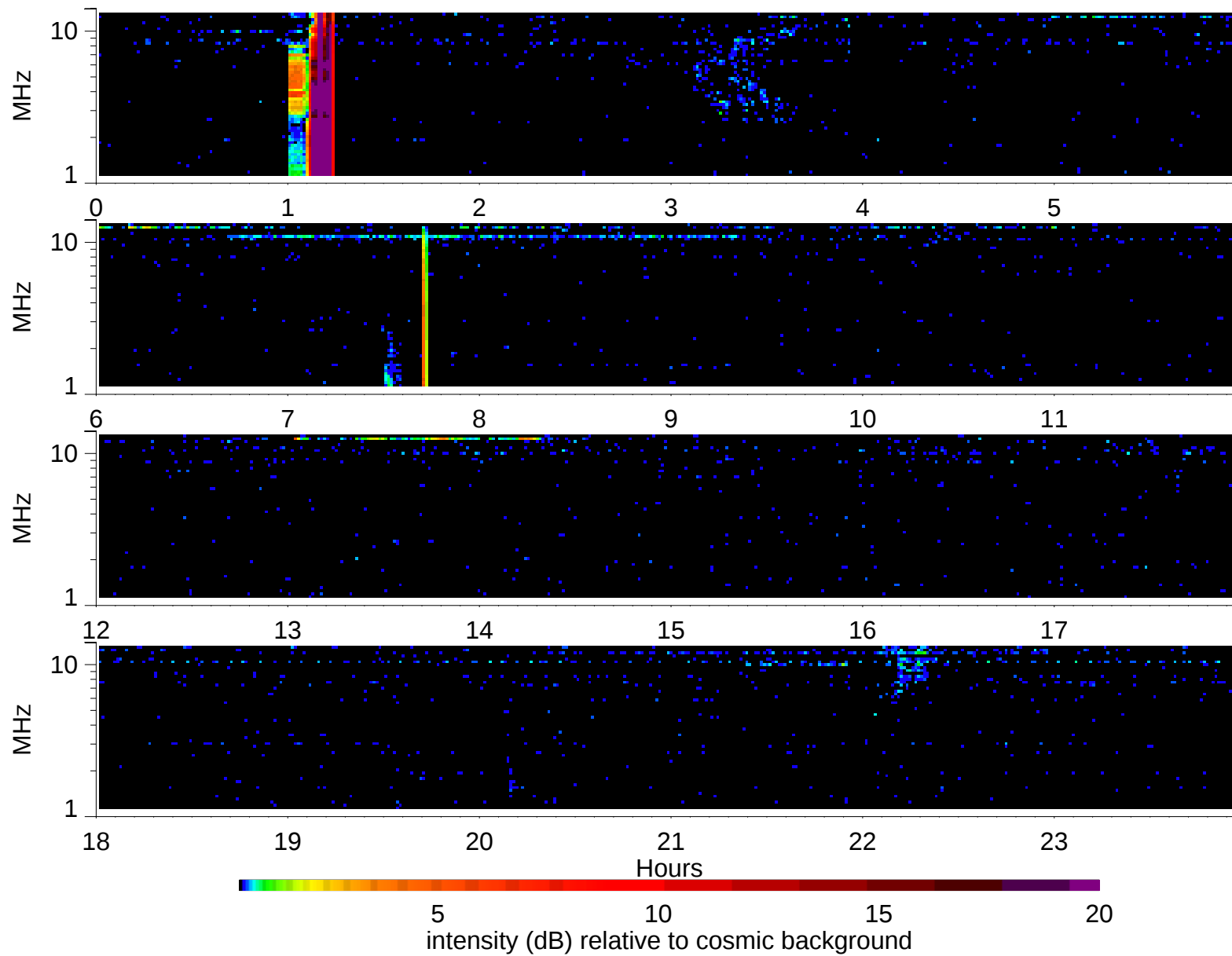
Wind Waves RAD2 receiver: 1998/1/8
