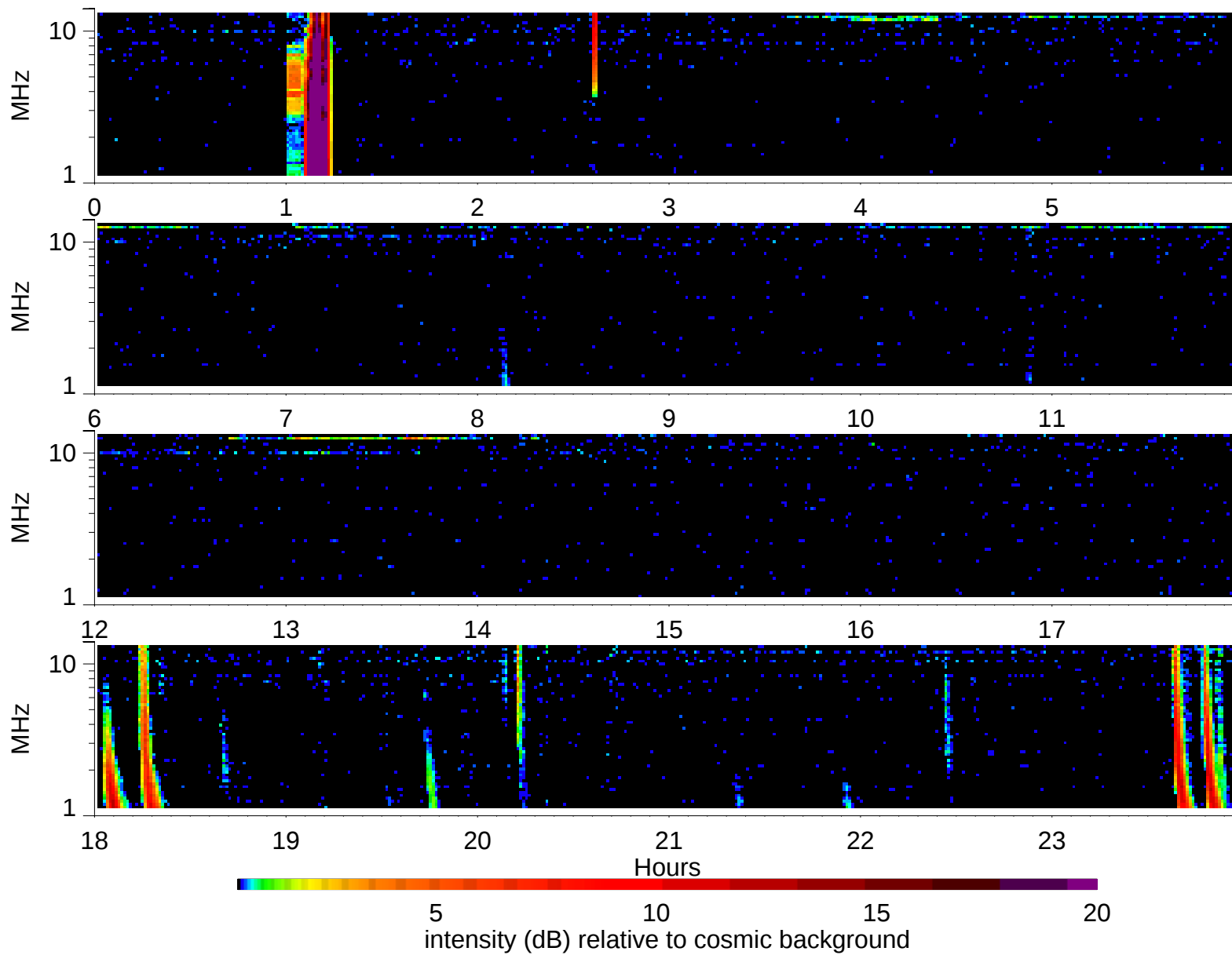
Wind Waves RAD2 receiver: 1998/1/10
