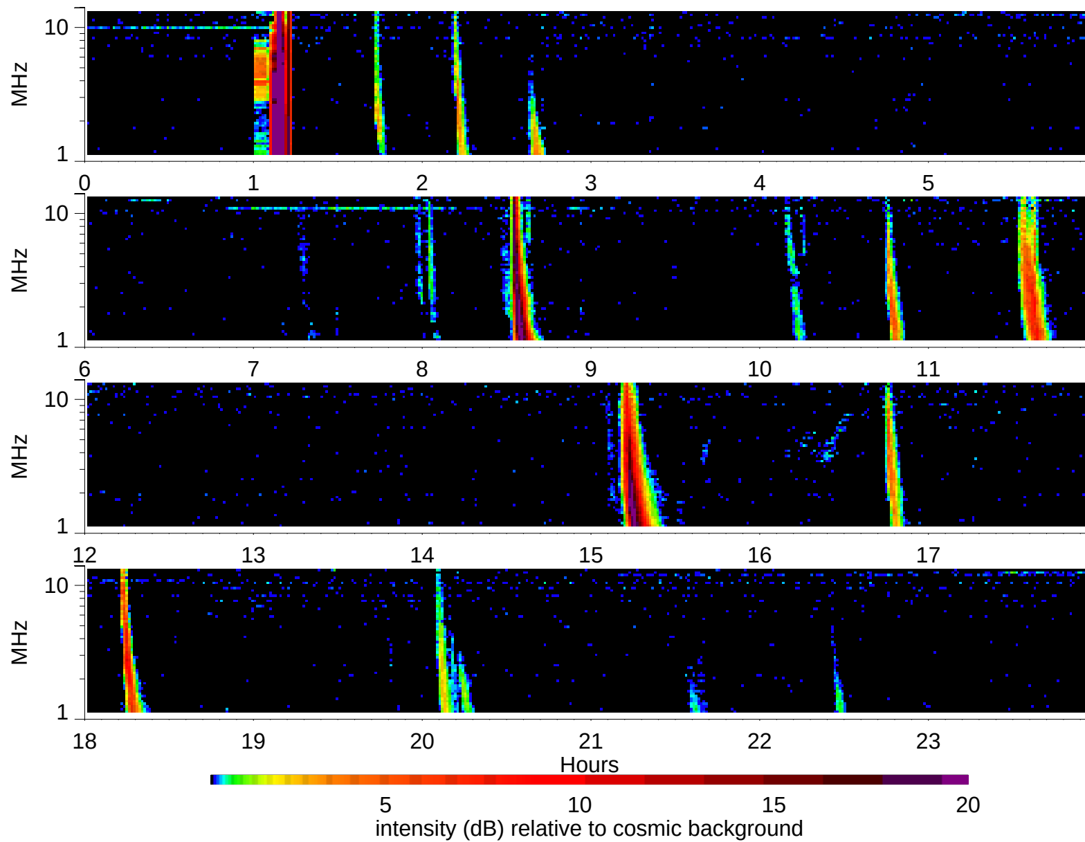
Wind Waves RAD2 receiver: 1998/1/12
