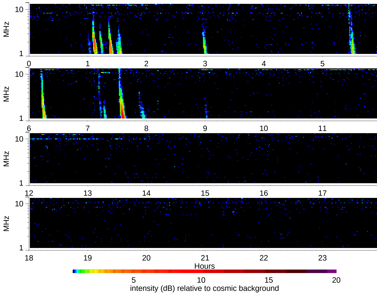
Wind Waves RAD2 receiver: 1998/1/23
