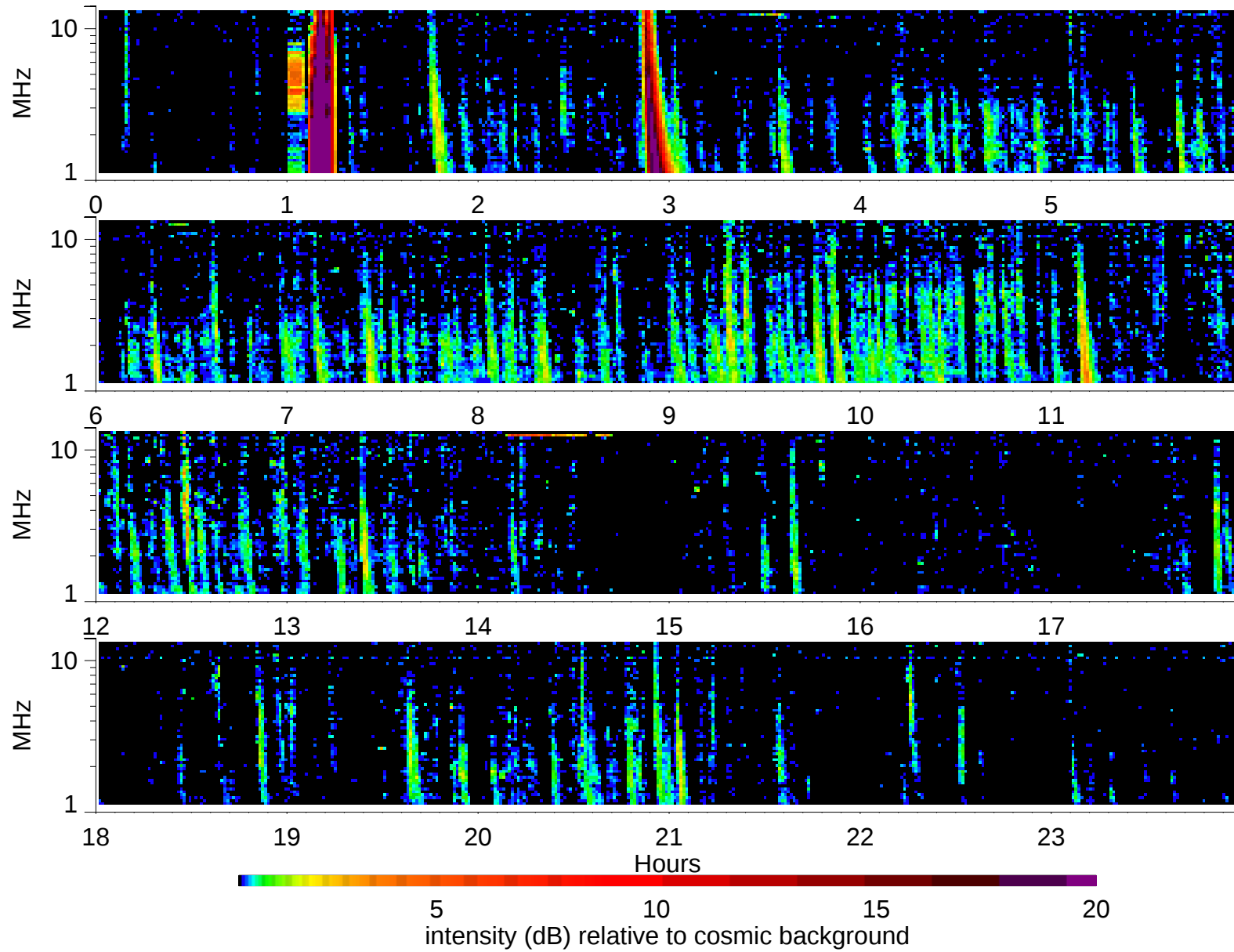
Wind Waves RAD2 receiver: 1998/1/28
