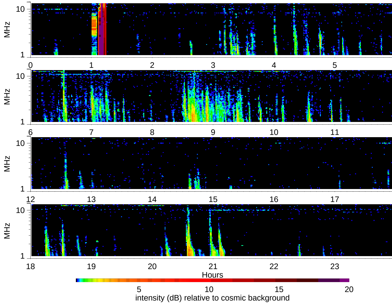
Wind Waves RAD2 receiver: 1998/1/30
