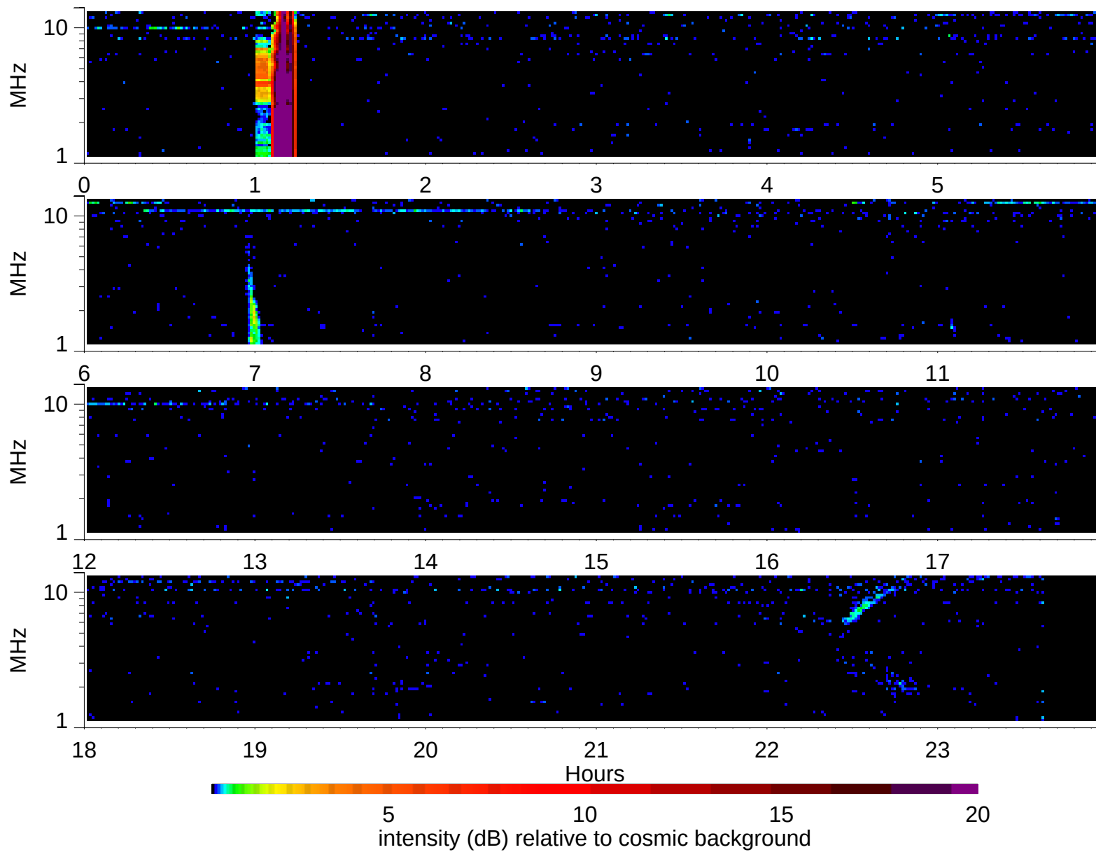
Wind Waves RAD2 receiver: 1998/2/1
